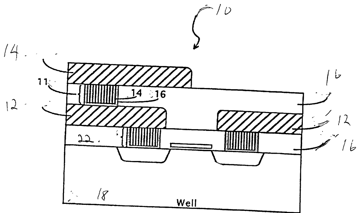
Figure 1 (Prior Art)
